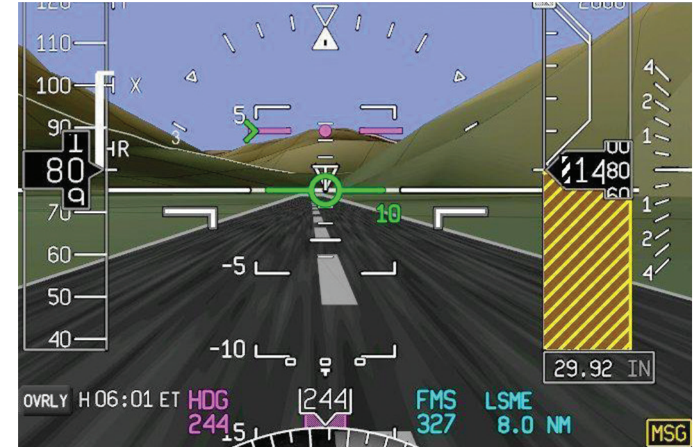
Approach with extended center-line, provided by the SmartView™ Synthetic Vision System, increases position awareness with respect to the landing environment.
